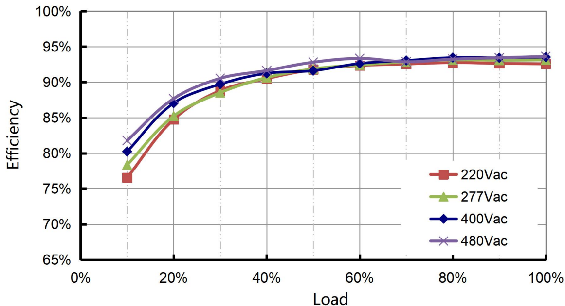
Efficiency vs. Load (C210)
